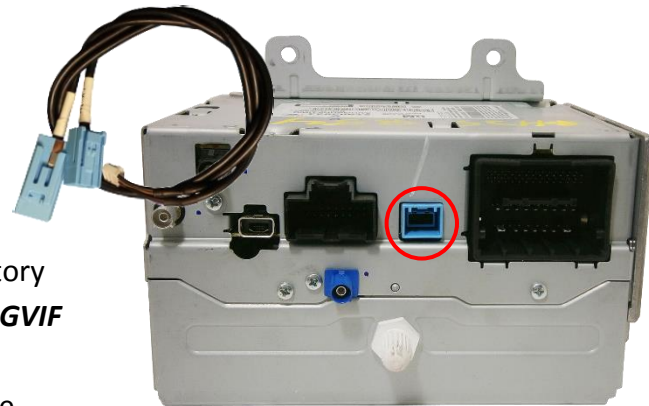
OEM GVIF Radio
